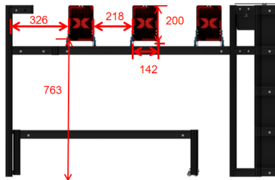
Fig 4.2-8 Reversed Flag Area(Front View)
