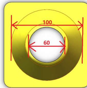
Fig 4.3-9 Cone(Top View)
